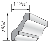
3" Crown VER52
