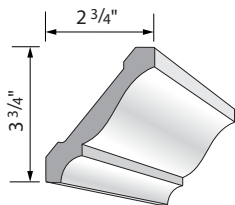
5" Crown VER47
