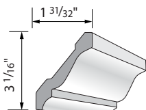
4" Crown VER49
