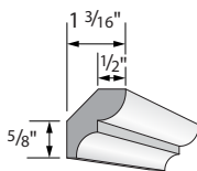
Bed Mould VER75
