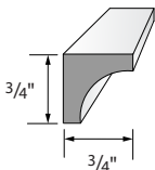
Scotia Cove VER93
