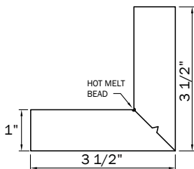
Regular Corner | Nominal 5/4 x 4 Profile
