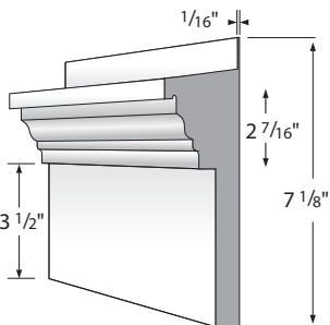
Crosshead Pediment VERCHP01
