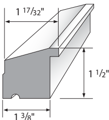
Sub Sill Nose VER282
