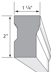
Brick Mould VER180 ■ 18'
