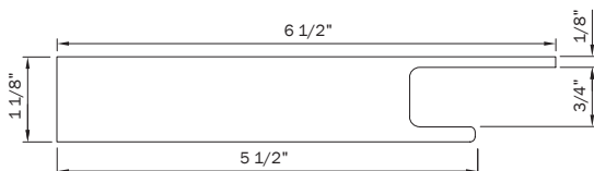
Stealth Casing with J-Channel | Nominal 5/4 x 6 Profile
