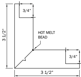
Stealth Corner Nominal 5/4 x 4 Profile
