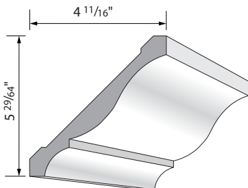
8" Crown PA8CROWN
