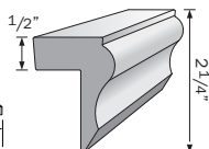
Beadboard Cap PABEADCAP
